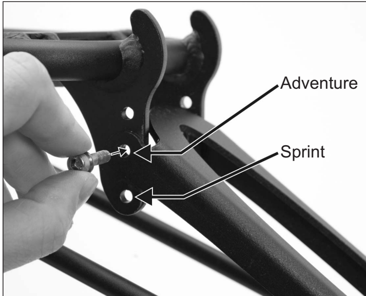
Assemble rack by bolting the front plate to the rack top using through the correct holes for your trike. Use M5 x 16 bolt and nut on each side.
